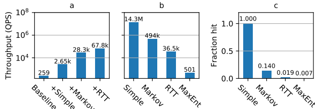
Figure 13: Cascades in MacroBase: (a) as we incrementally add cascade stages, threshold query throughput increases. (b) The cascade proceeds from faster to slower estimates. (c) Each stage of the cascade processes a smaller fraction of queries.
