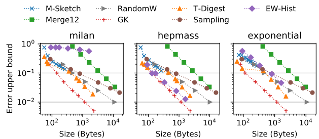
Figure 23: Average bound size for summaries of different sizes. No summary is able to provide \epsilon_{bound} \leq .01 guarantees with less than 1000 bytes.
