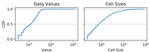
Figure 21: Microsoft data values and cell sizes.
