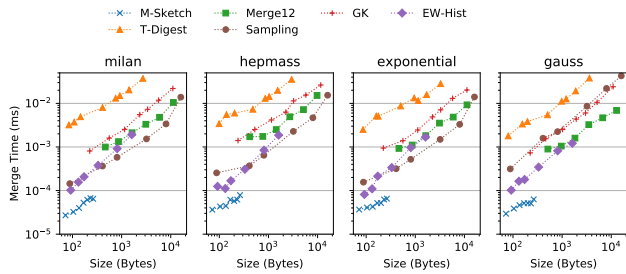
Figure 20: Merge times on sketches on cells of 2000 elements, and on a Gaussian dataset with cells of 10000 elements. Since the moments sketch has a fixed size, its per-merge times remain faster than alternative sketches with comparable accuracy.
