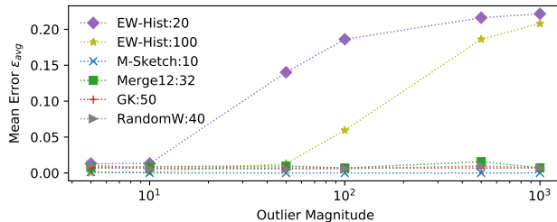
Figure 19: Mean error on a Gaussian dataset with outliers of different magnitudes added. The moments sketch remains accurate for large outliers, but the EW-Hist accuracy degrades.
