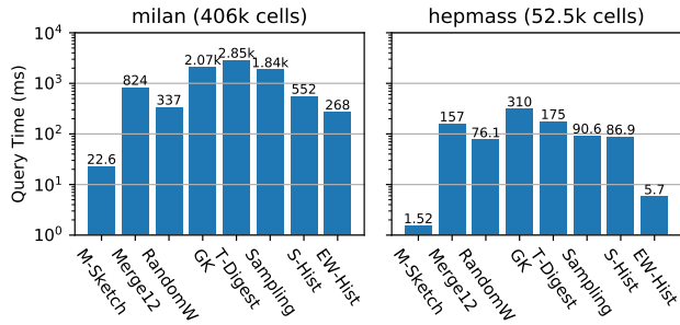
Figure 3: Total query time using different summaries to estimate quantiles with \epsilon_{\text{avg}} < .01 . The moments sketch enables significantly faster queries at this accuracy.
