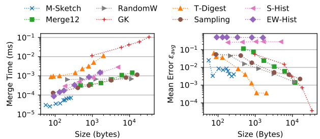
Figure 22: Merge times and accuracy on the Microsoft dataset. The merge performance of the moments sketch generalizes to workloads with variable sized cells, and exhibits an error rate of \epsilon_{avg} < .01 .
