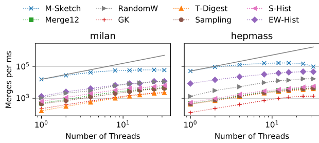
Figure 24: Strong scaling of parallel merging. For fixed number of merges, the throughput of the moments sketch scales with the number of threads available up to 8-way parallelism, and remains faster than alternatives. The solid line shows ideal moments sketch scaling.
